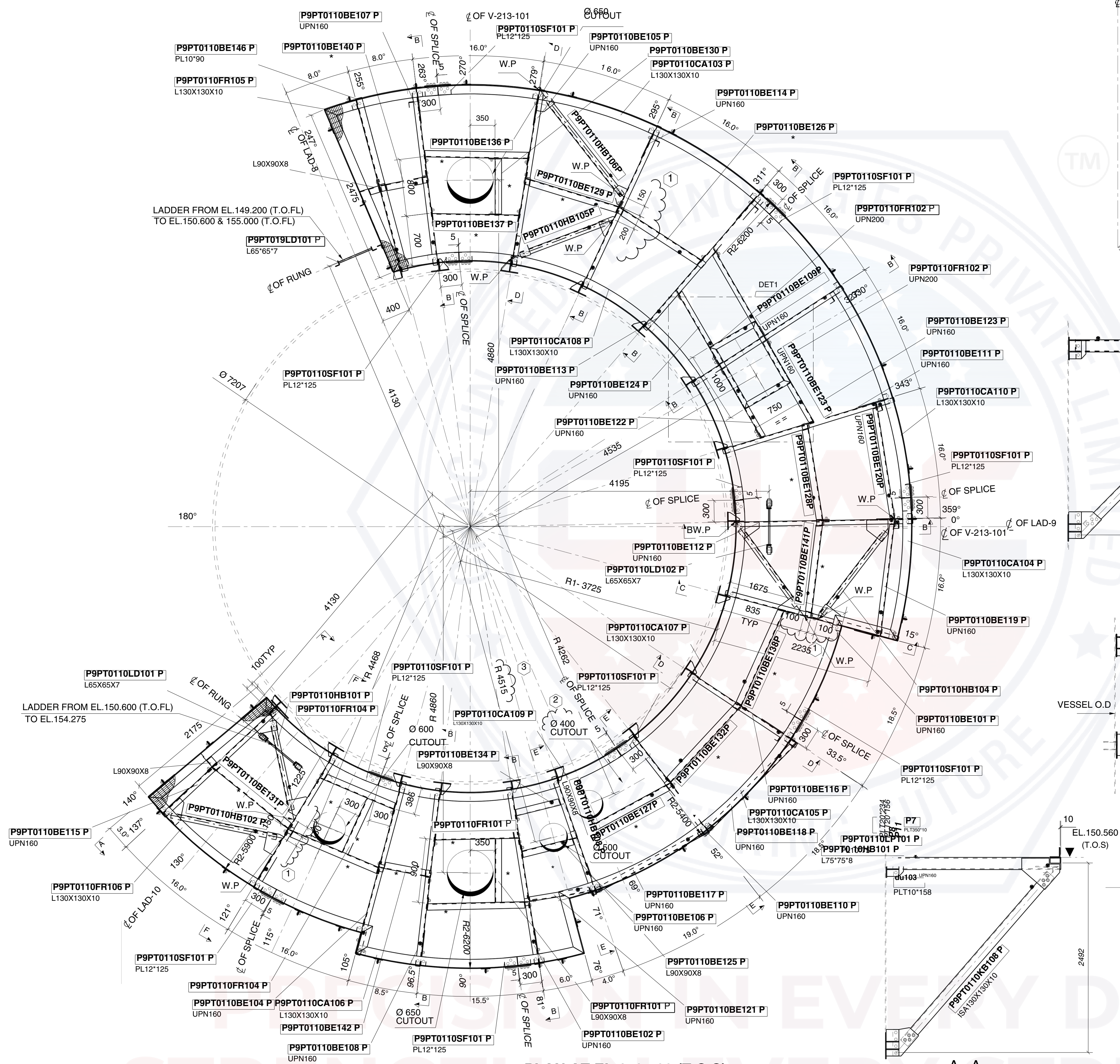
PLAN AT EL.150.560 (T.O.S) ALL PLAN BRACINGS ARE L75X75X8 (-125) FROM (T.O.S) (U.O.N) MEMBER MARKED *** ARE L90X90X8 (+10) FROM (T.O.S) (U.O.N) (PLATFORM TOP AT EL.150.600)
