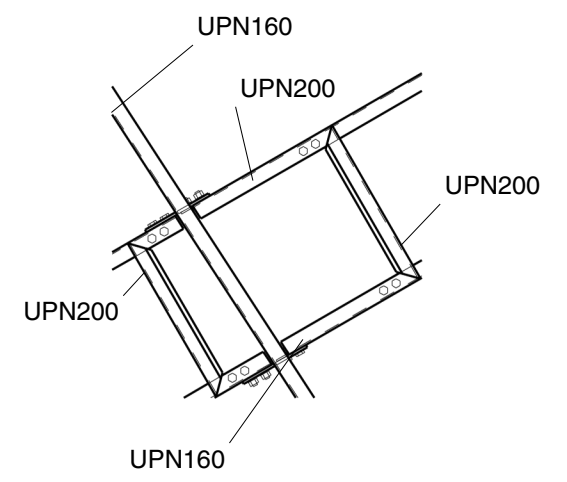
DETAIL-2
