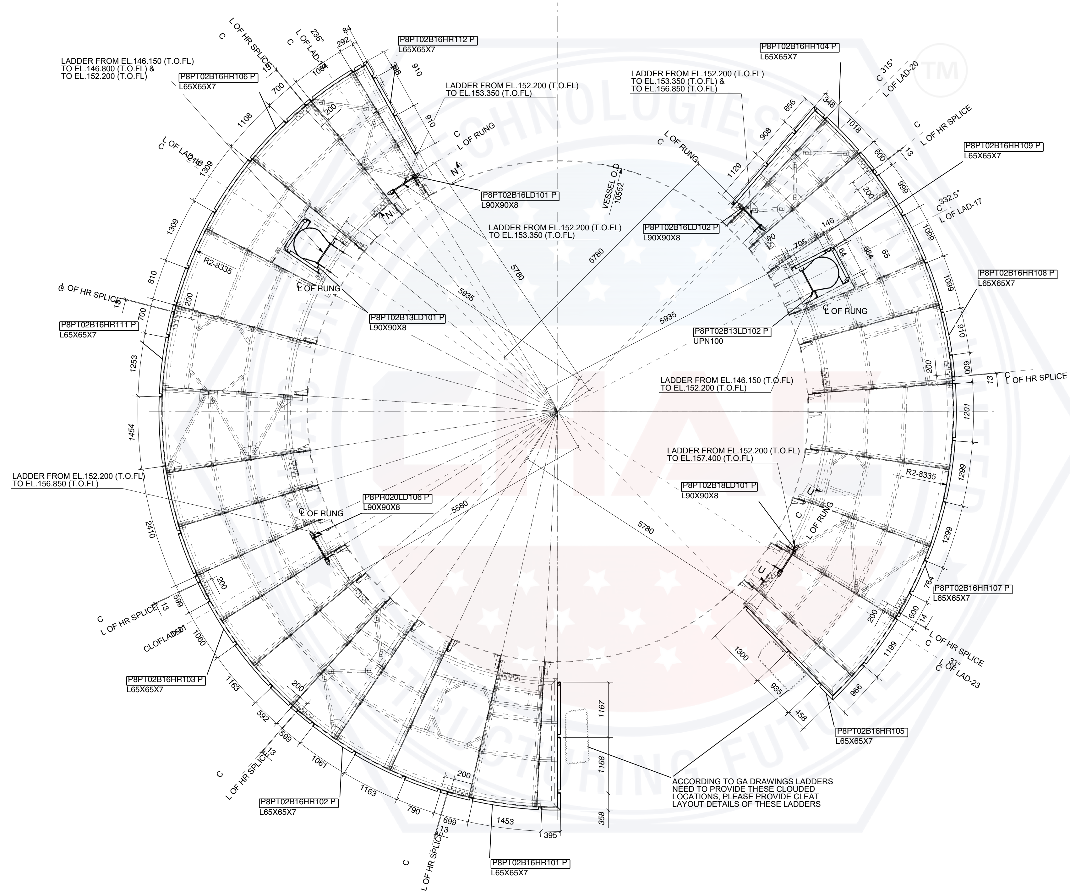
HANDRAIL PLAN AT EL.152.000(T.O.S)
